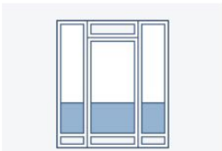
Single Door 2 Panel and Transom Width 48" to 124"
